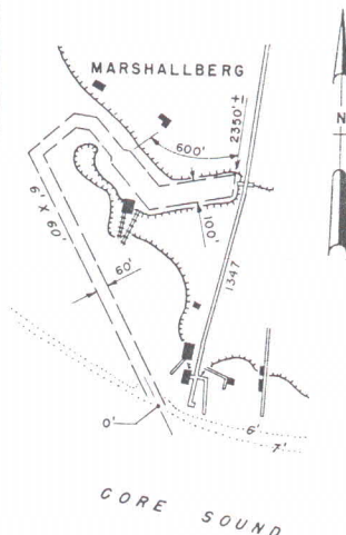
DETAIL OF BASIN SCALE OF FEET 0 200 400 600 800
